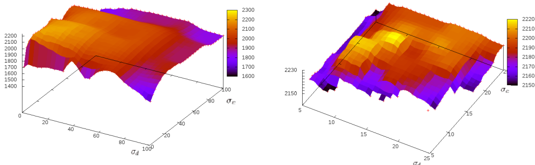
Figure 10: Score in the challenge against \sigma_d and \sigma_c . Figure 11: Zoom on the best scores in the challenge against \sigma_d and \sigma_c .
